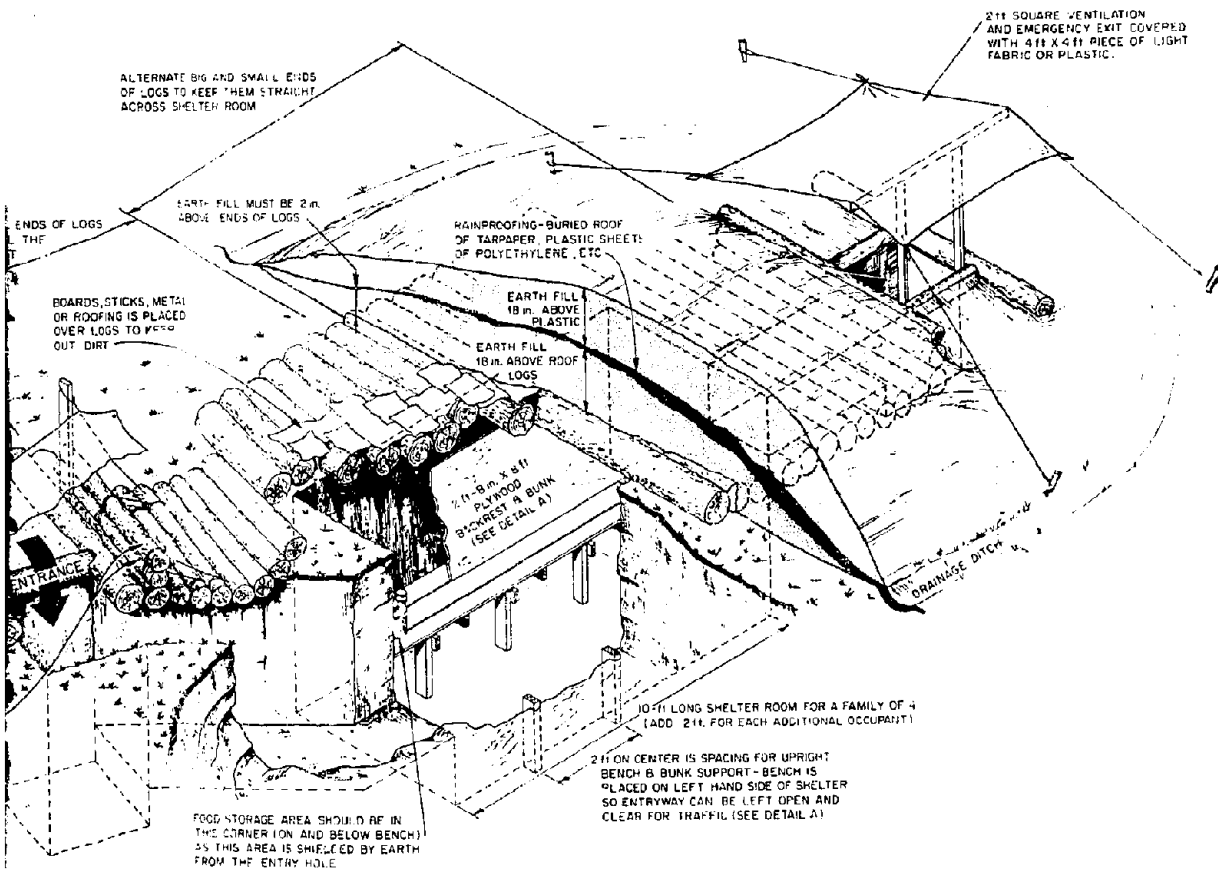
Covered Trench Shelter, Pictorial View.
